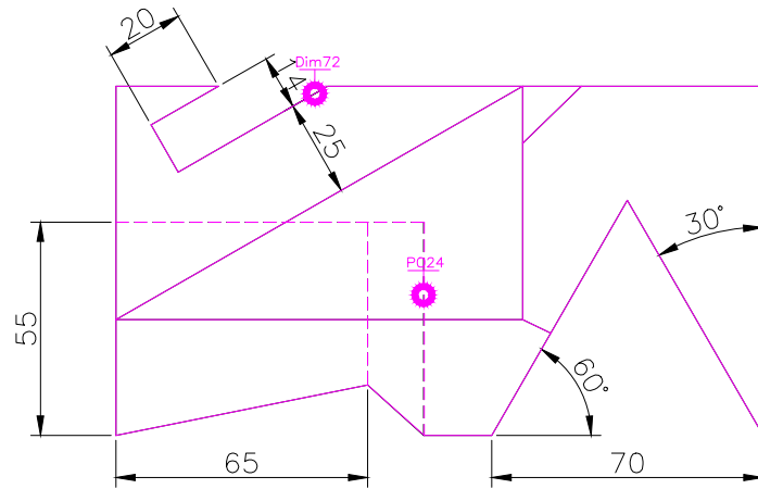
TOP SCALE 1/2
