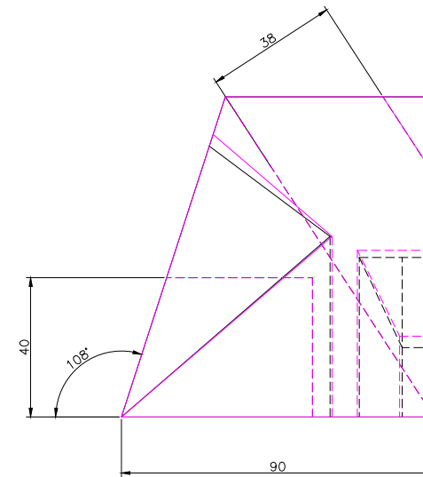
RIGHT SCALE 1/2
