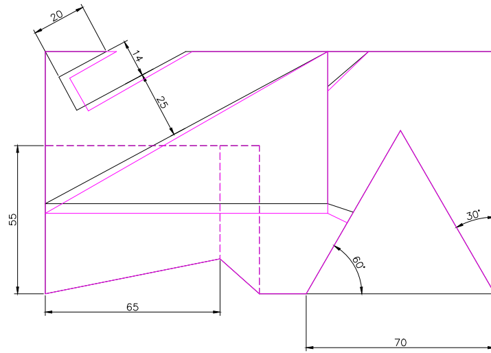
TOP SCALE 1/2
