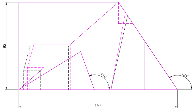
FRONT SCALE 1/2
