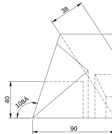
RIGHT SCALE 1/2
