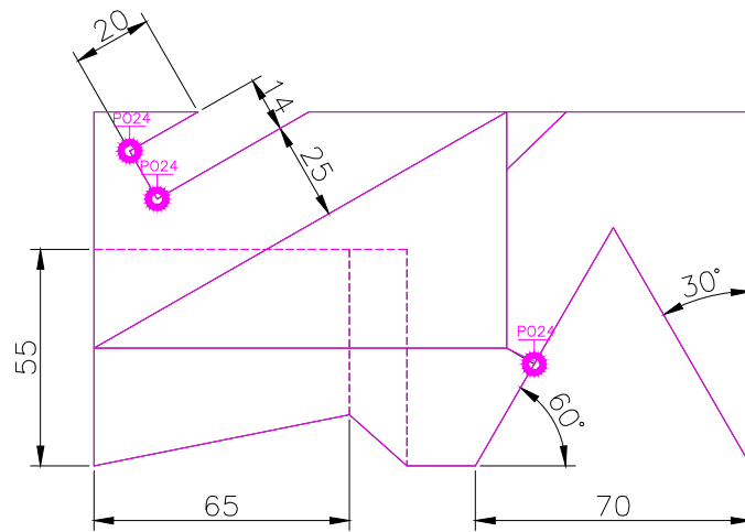
TOP SCALE 1/2
