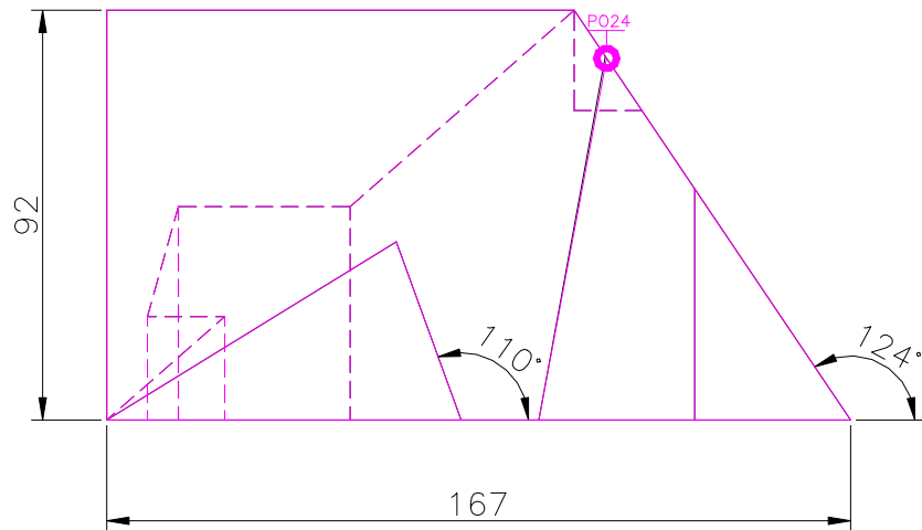
FRONT SCALE 1/2
