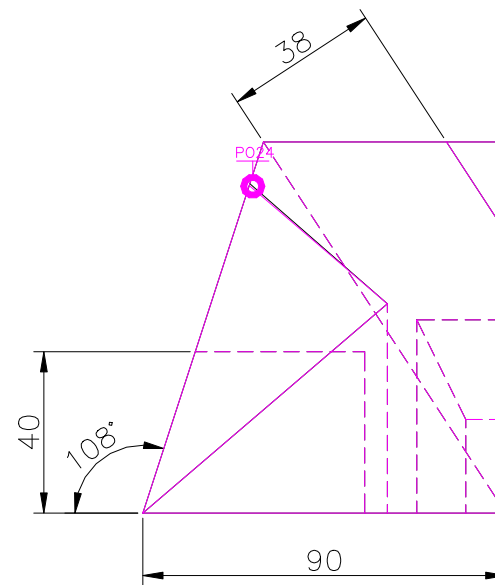
RIGHT SCALE 1/2
