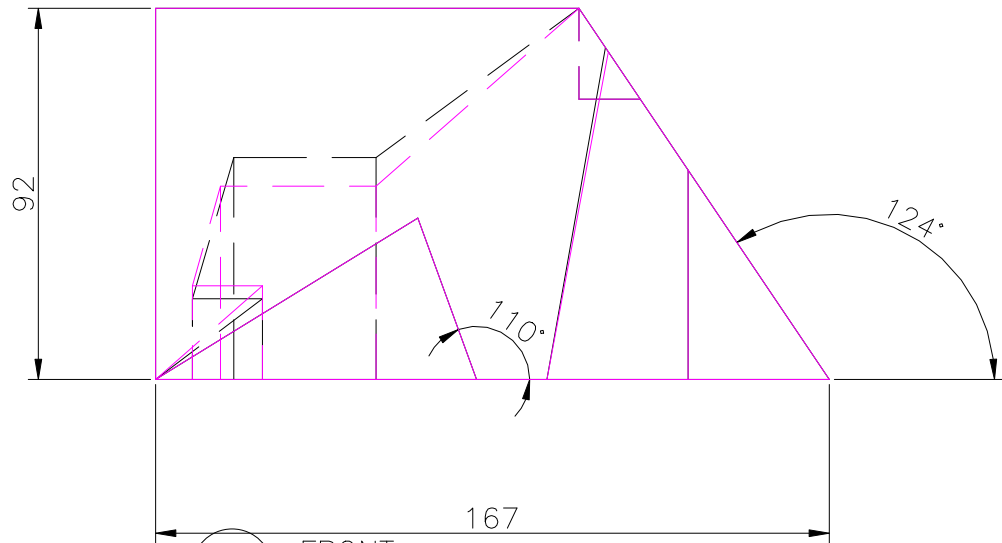
FRONT SCALE 1/2
