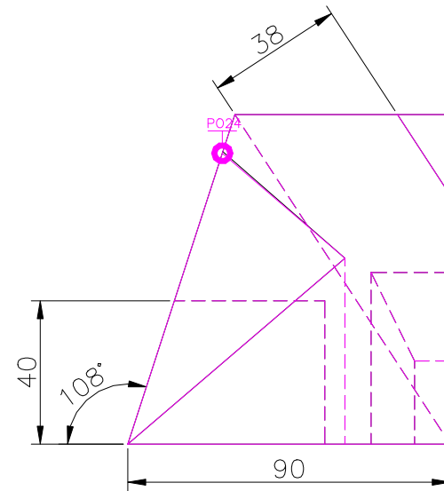
RIGHT SCALE 1/2
