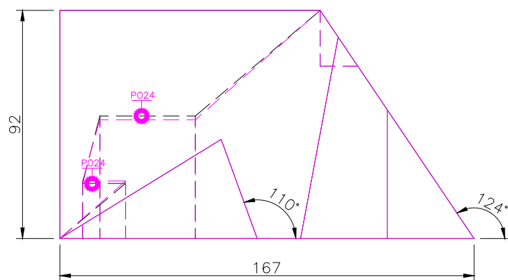
FRONT SCALE 1/2
