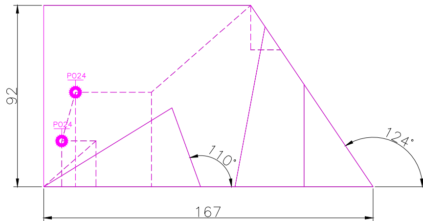
FRONT SCALE 1/2
