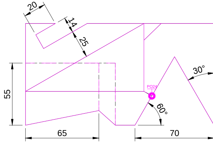
TOP SCALE 1/2
