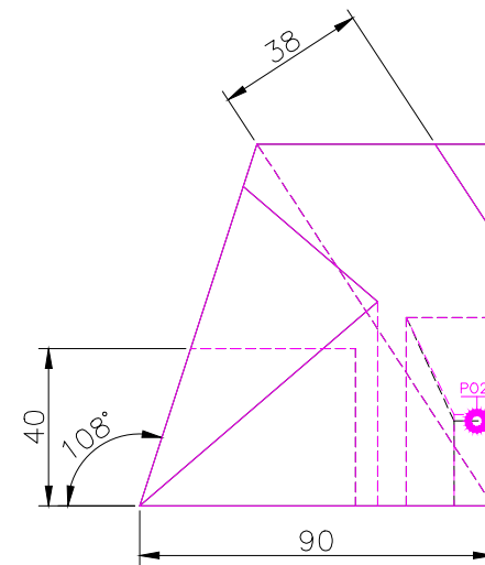
RIGHT SCALE 1 / 2
