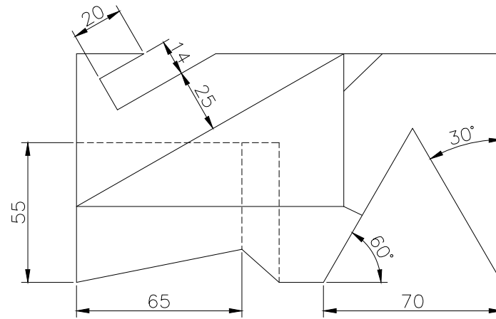
TOP SCALE 1 / 2
