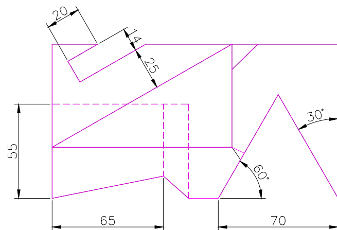
TOP SCALE 1/2
