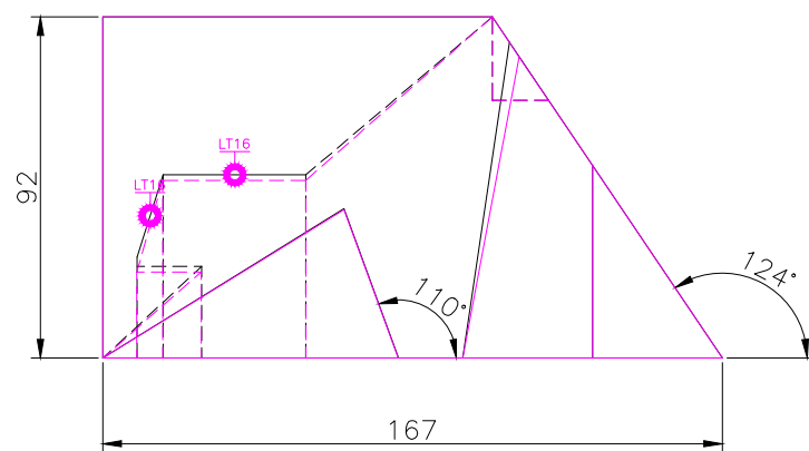
FRONT SCALE 1/2
