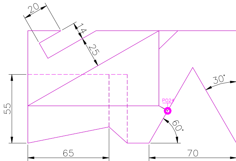
TOP SCALE 1/2
