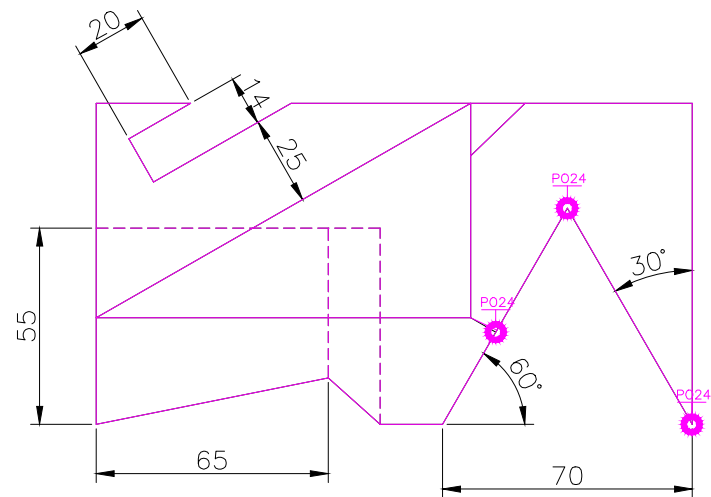
TOP SCALE 1/2
