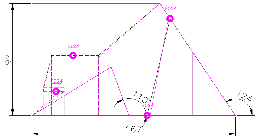
FRONT SCALE 1/2
