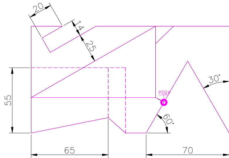
TOP SCALE 1/2
