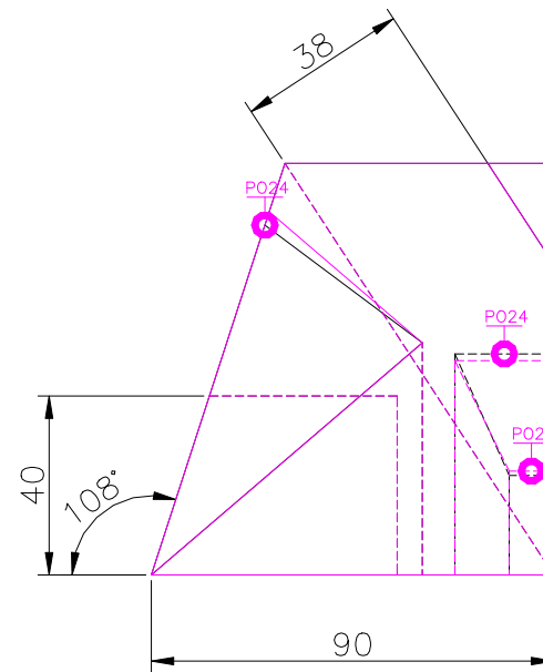
RIGHT SCALE 1/2
