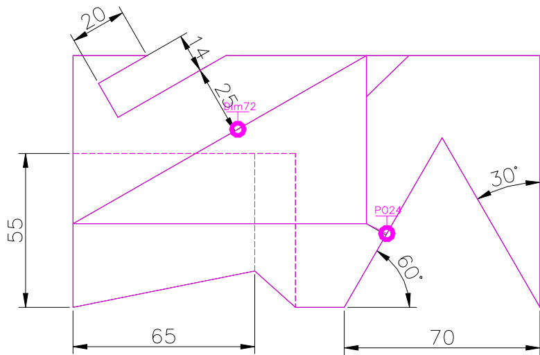
TOP SCALE 1/2
