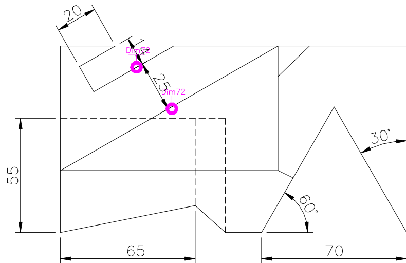
TOP SCALE 1/2
