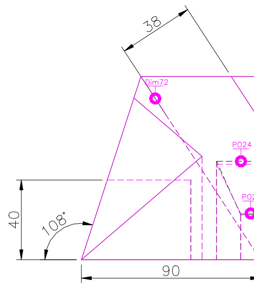
RIGHT SCALE 1/2
