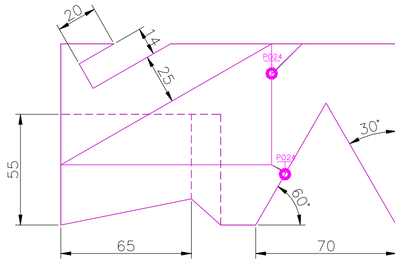
TOP SCALE 1/2
