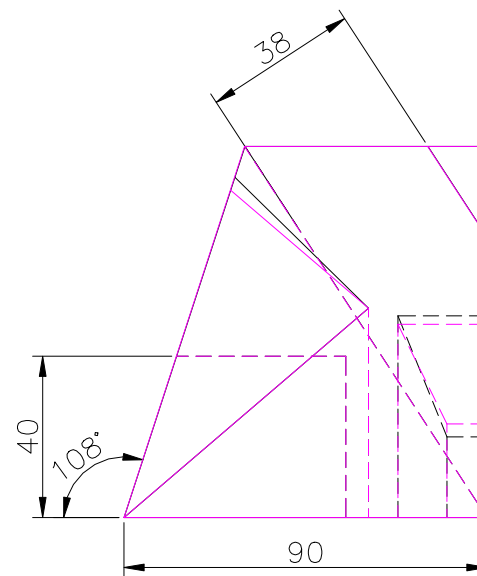
RIGHT SCALE 1/2
