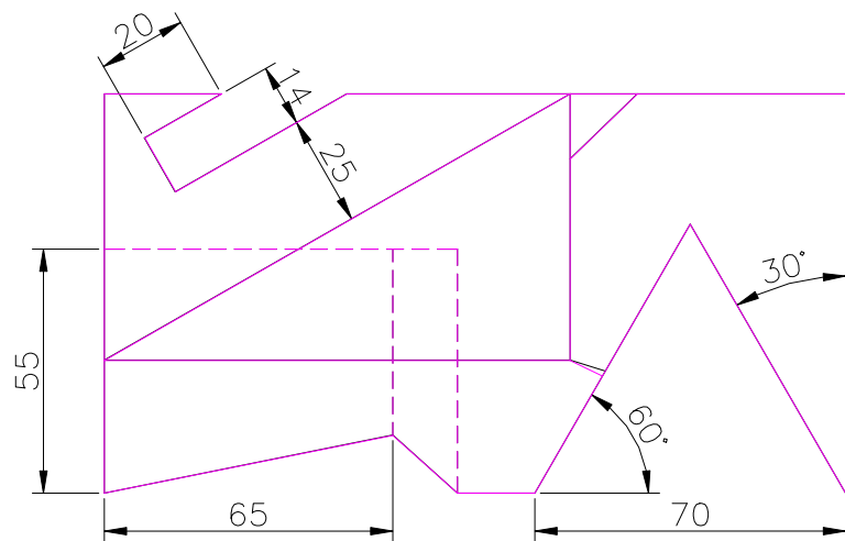
TOP SCALE 1/2
