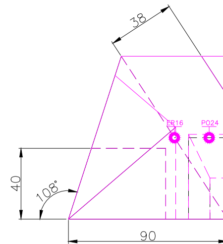
RIGHT SCALE 1/2
