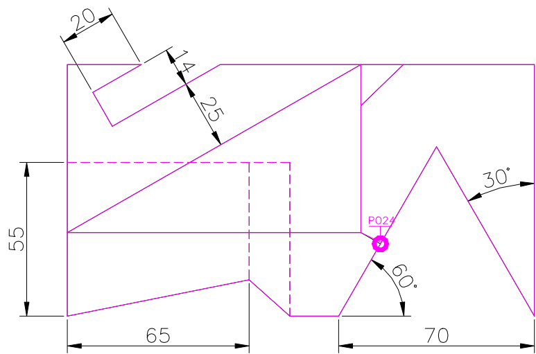
TOP SCALE 1/2
