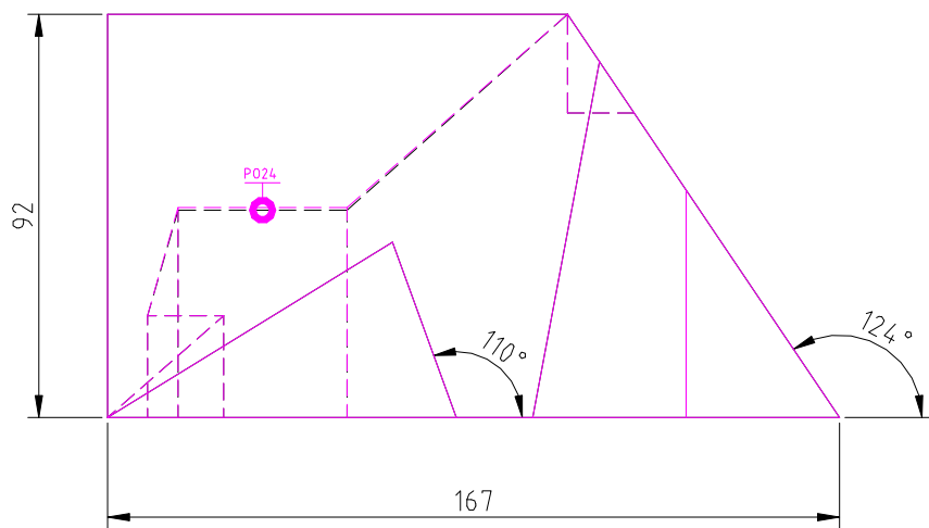
FRONT SCALE 1/2
