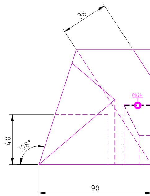
RIGHT SCALE 1/2
