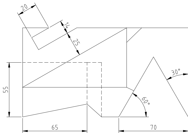
TOP SCALE 1/2
