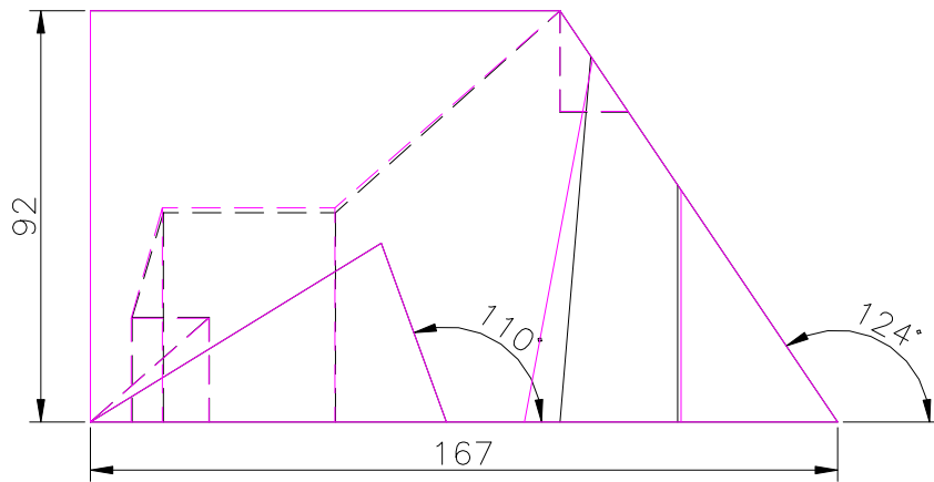
FRONT SCALE 1/2
