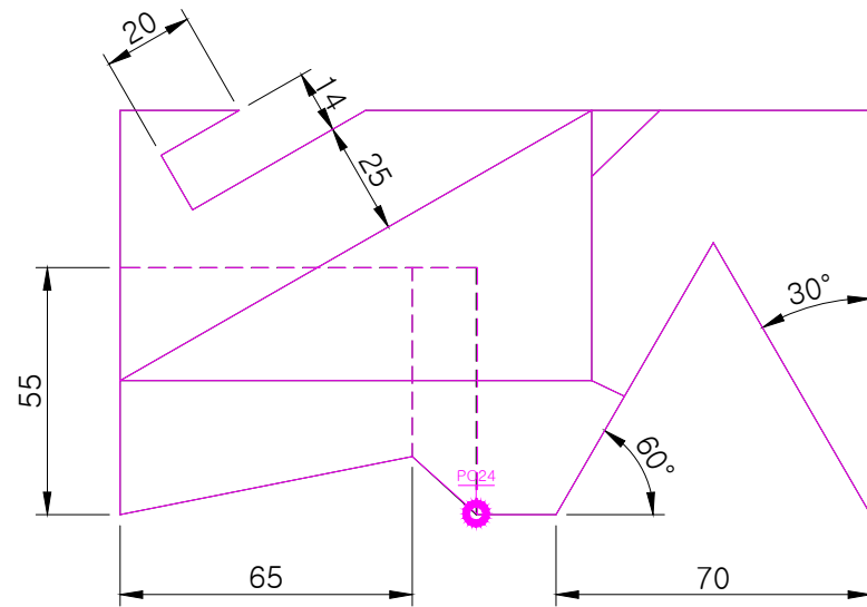
TOP SCALE 1/2
