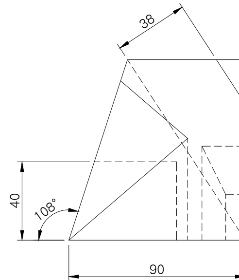
RIGHT SCALE 1/2
