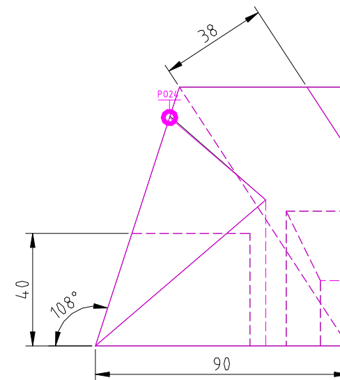
RIGHT SCALE 1/2
