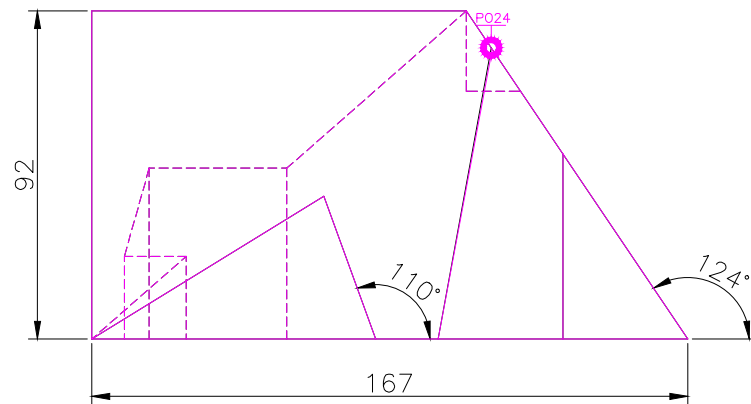
FRONT SCALE 1/2
