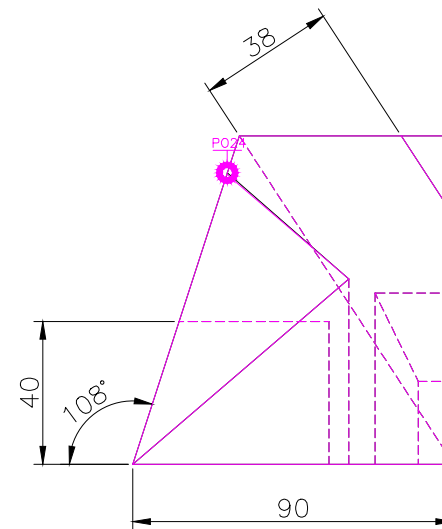
RIGHT SCALE 1/2
