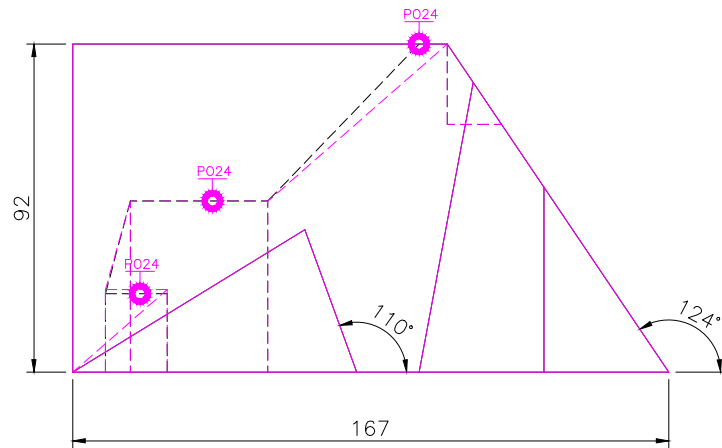
FRONT SCALE 1/2
