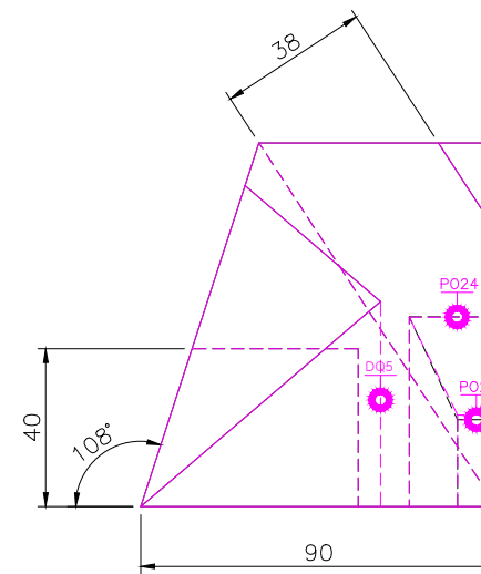
RIGHT SCALE 1/2
