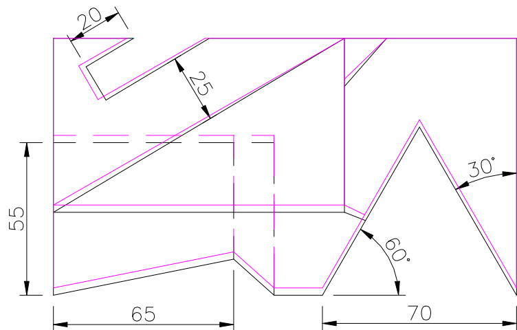
TOP SCALE 1/2
