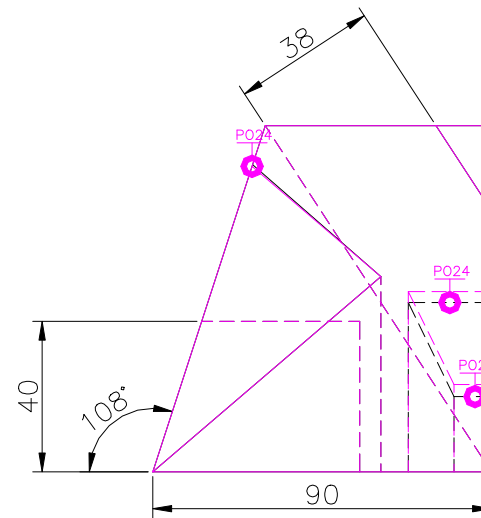
RIGHT SCALE 1/2
