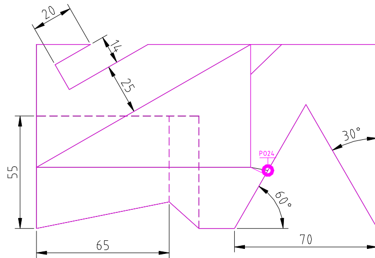
TOP SCALE 1/2
