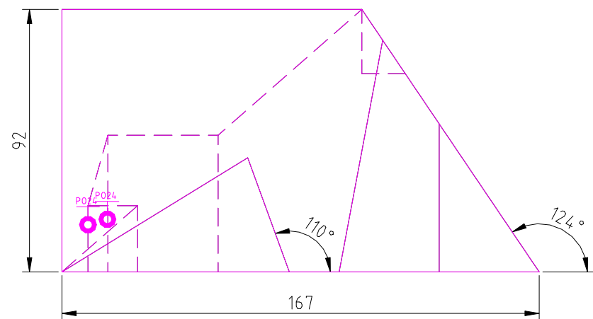
FRONT SCALE 1/2
