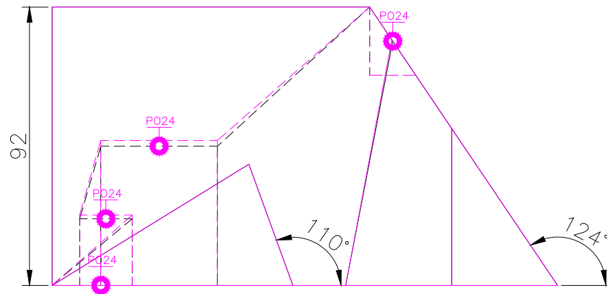
FRONT SCALE 1/2
