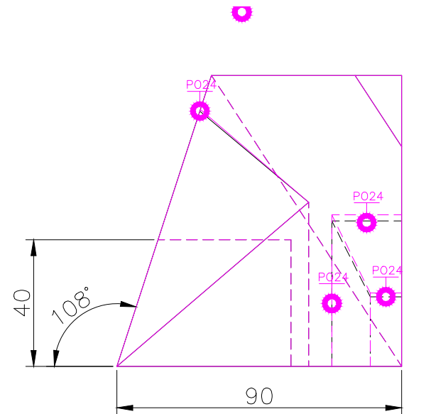
RIGHT SCALE 1/2
