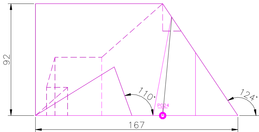
FRONT SCALE 1/2
