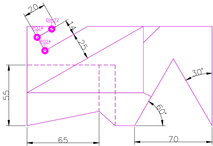
TOP SCALE 1/2
