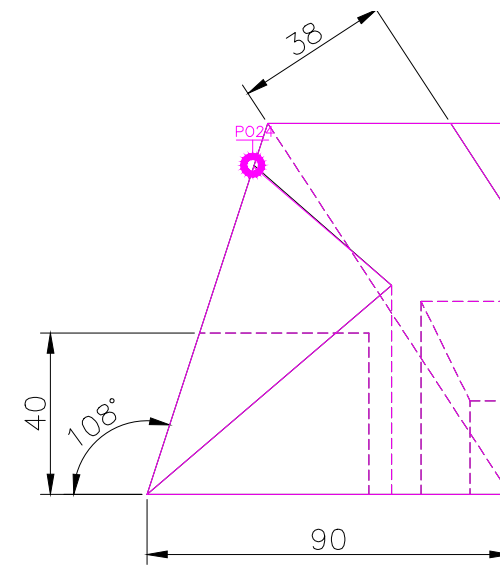
RIGHT SCALE 1/2
