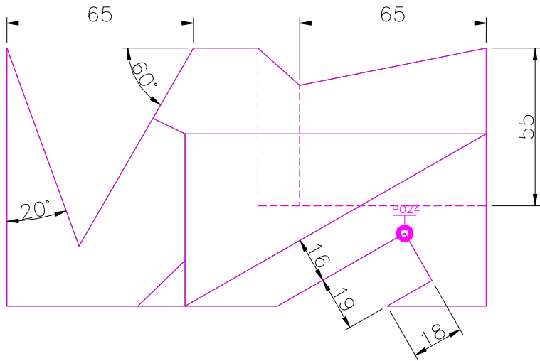
TOP SCALE 1/2
