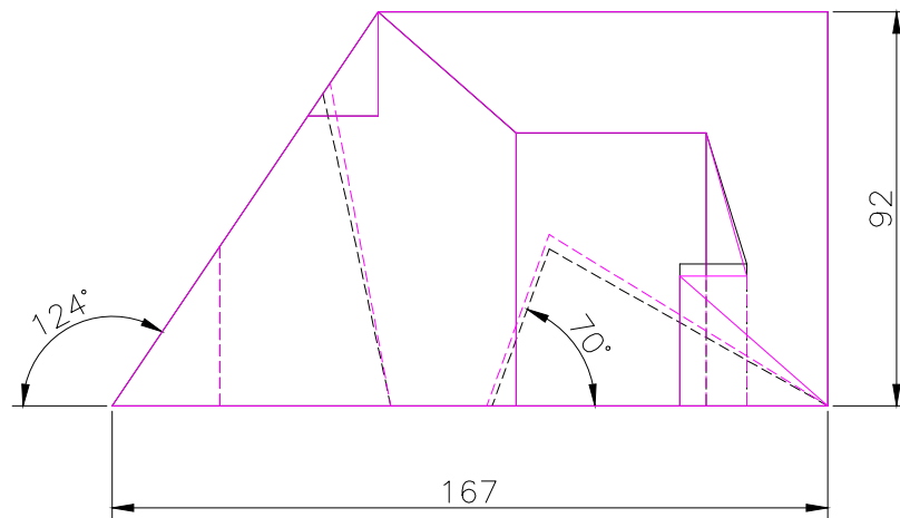
FRONT SCALE 1/2
