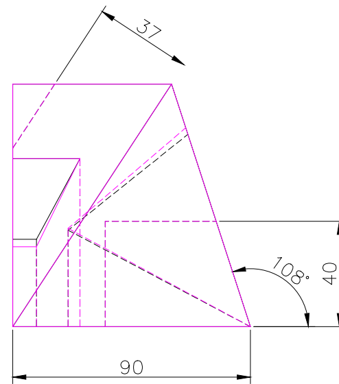
RIGHTT SCALE 1/2
