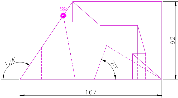
FORNT SCALE 1/2
