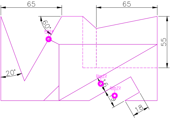
TOP SCALE 1/2
