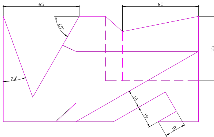
TOP SCALE 1/2
