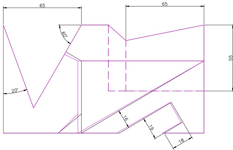
TOP SCALE 1/2
