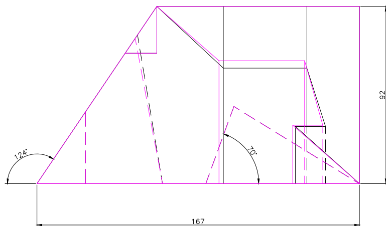
FRONT SCALE 1/2
