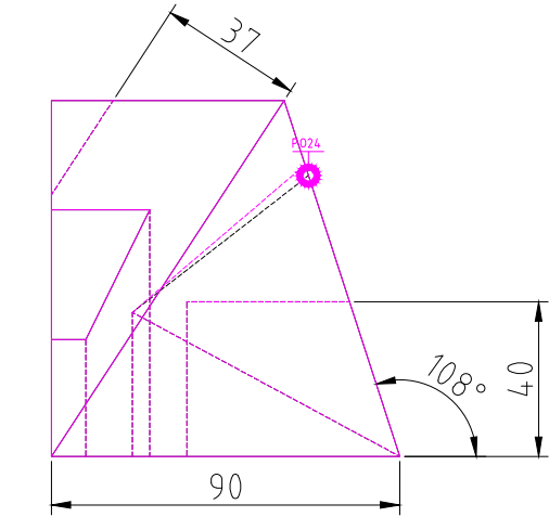
RIGHT SCALE 1/2
