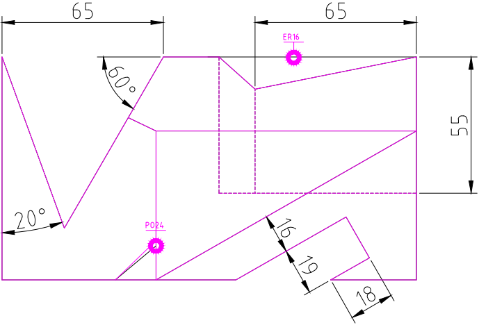
TOP SCALE 1/2
