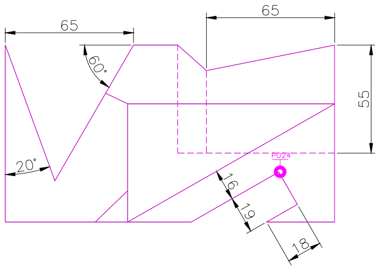
TOP SCAEL 1/2
