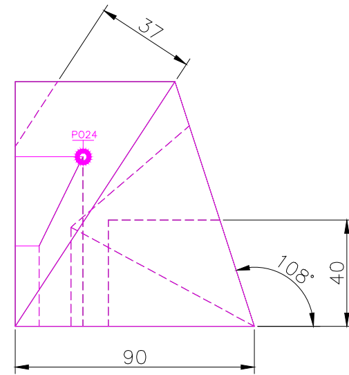
RIGHT SCAEL 1/2
