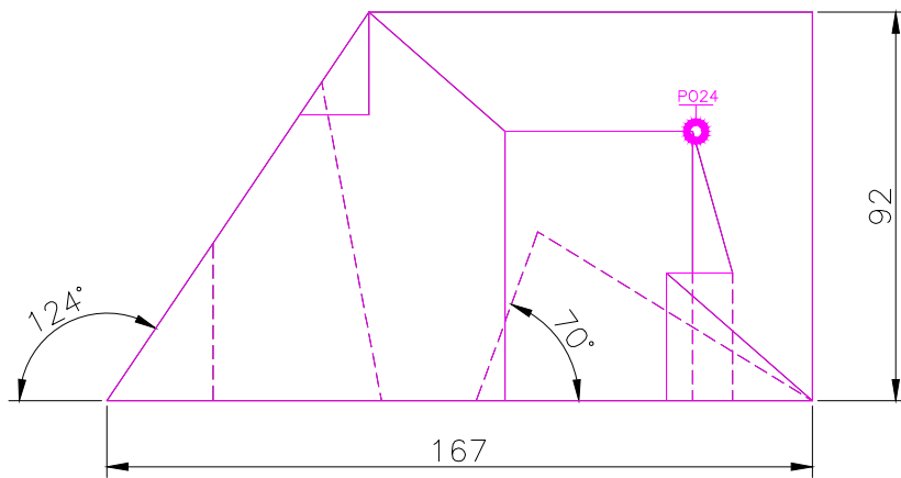
FRONT SCAEL 1/2
