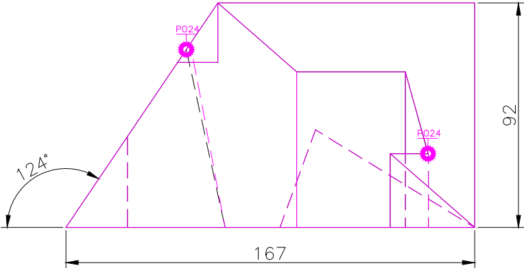
FRONT SCALE 1/2
