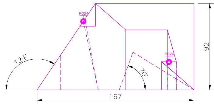
FRONT SCALE 1/2
