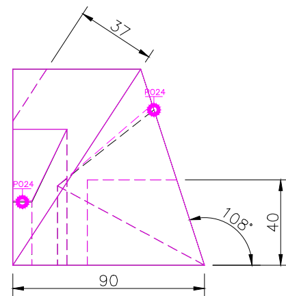
RIGHT SCALE 1/2
