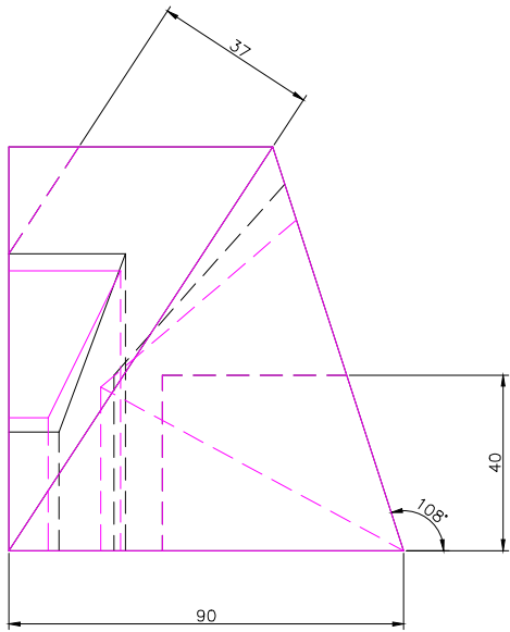
RIGHT SCALE 1/2
