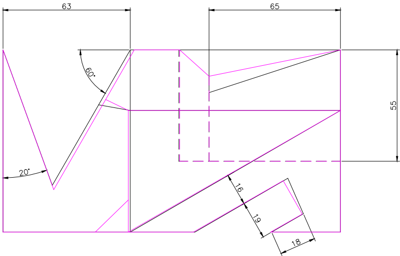
TOP SCALE 1/2
