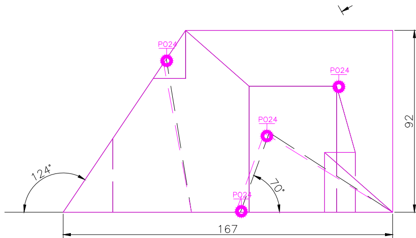
FRONT SCALE 1/2
