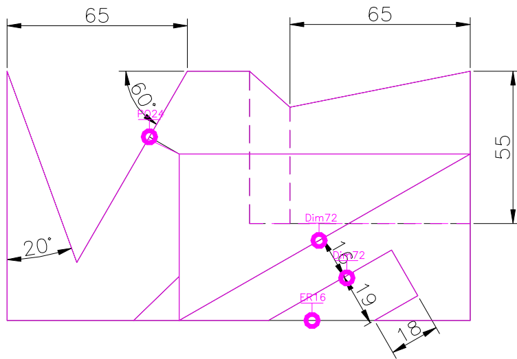
TOP SCALE 1/2
