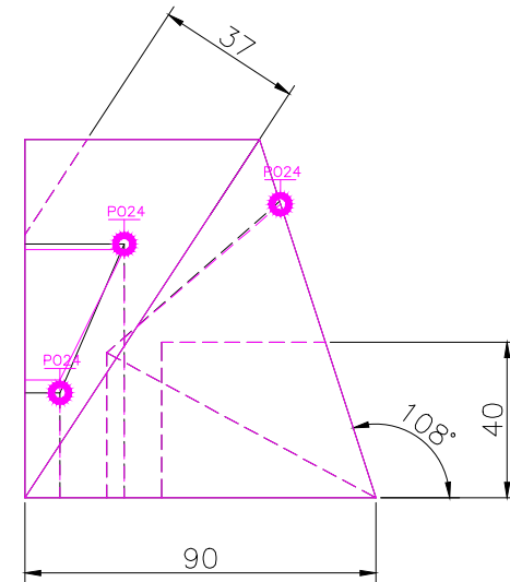
RIGHT SCALE 1/2
