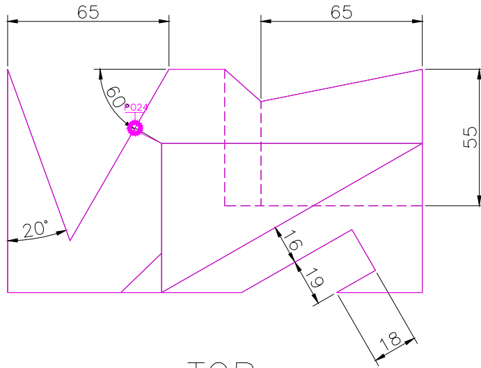
TOP SCALE 1/2
