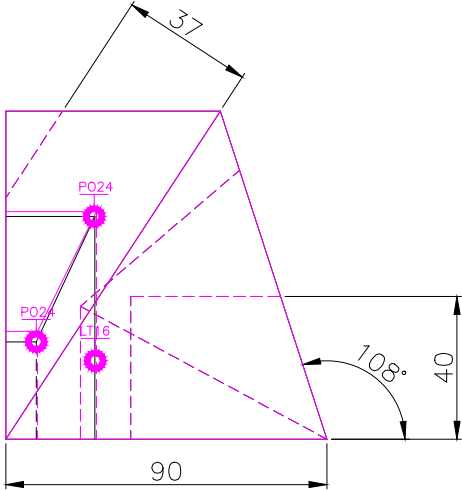
RIGHT SCALE 1/2
